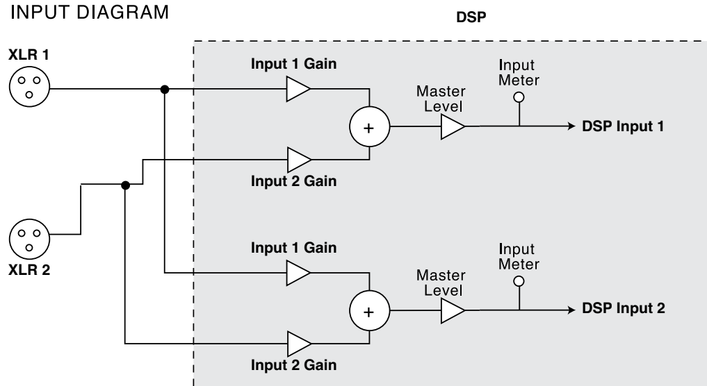
INPUT DIAGRAM
